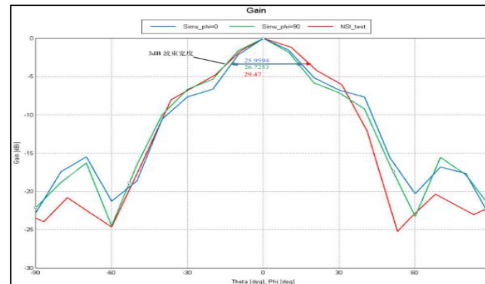
Near-field measurements
