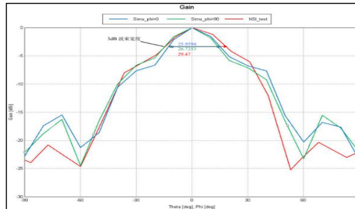
Near-field measurements
